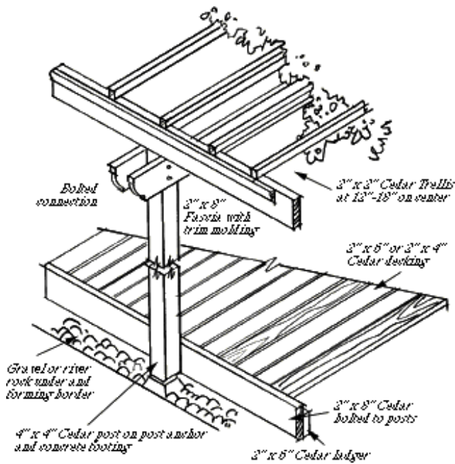
COVERED WALKWAY PLAN AND DETAIL
